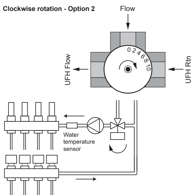
Figure C-1: Clockwise operation valve options
