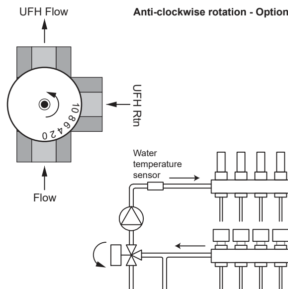
Anti-clockwise rotation - Option 3
