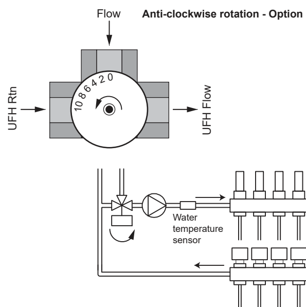
Figure C-2: Anti-clockwise operation valve options
