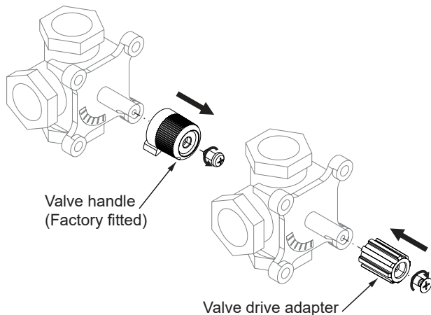
Figure C-3: Fitting the valve drive adapter
