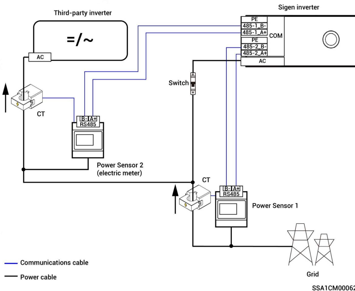
Figure 1. Diagram of third-party inverter wiring connections
