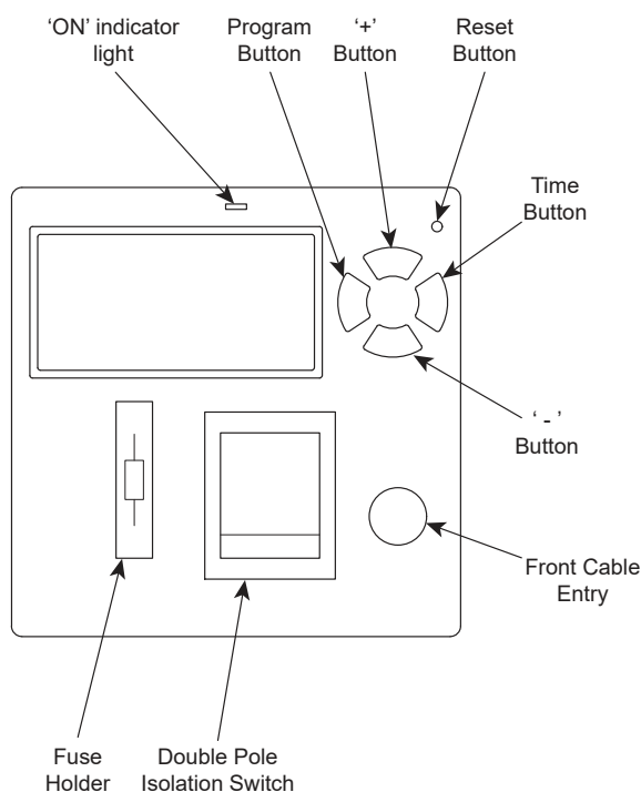
Figure 2: Greenbrook T205-C Fused Timer Spur Switch
